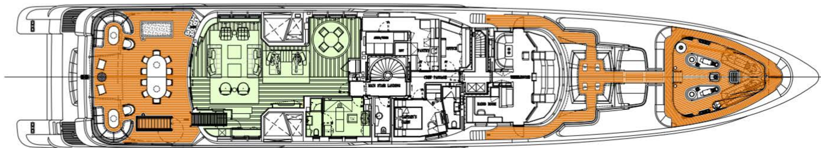
BRIDGE DECK
